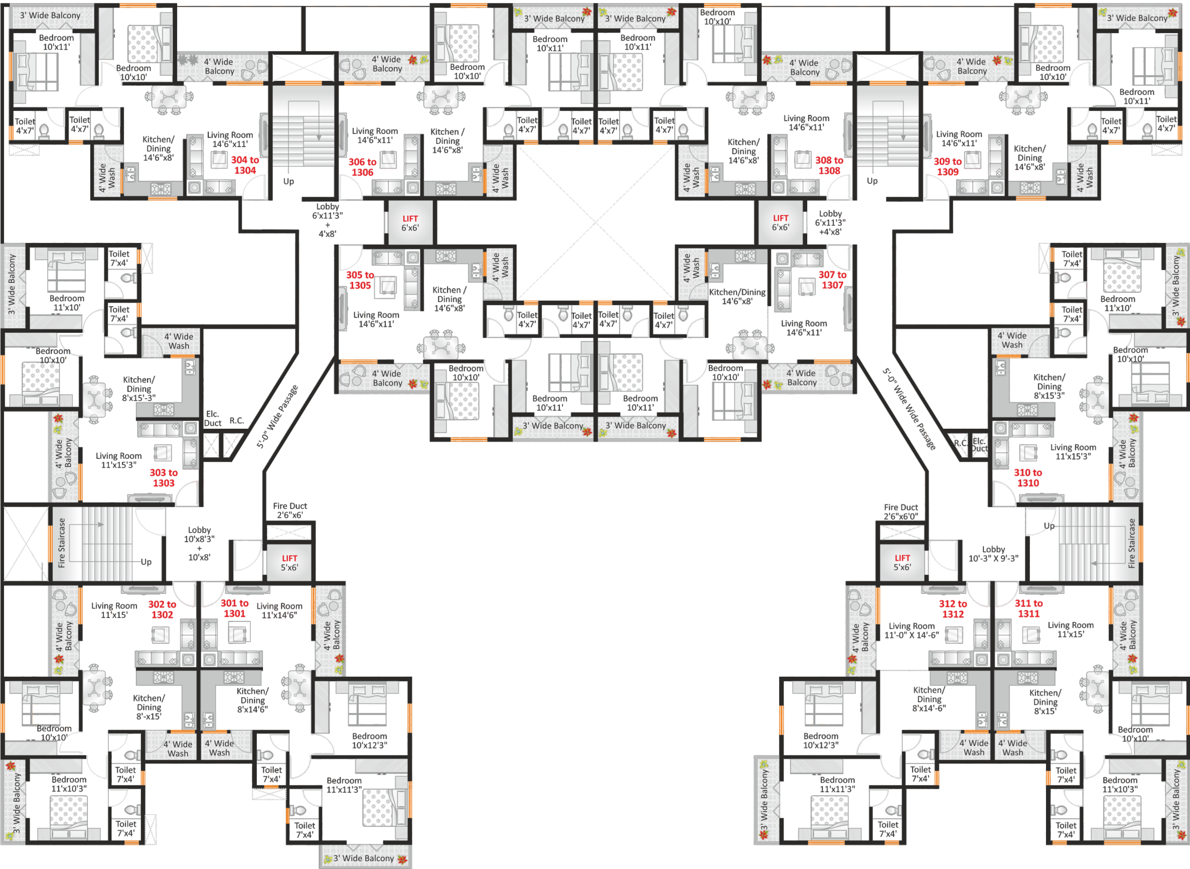
2BHK TYPICAL FLOOR PLAN - WING E & A
